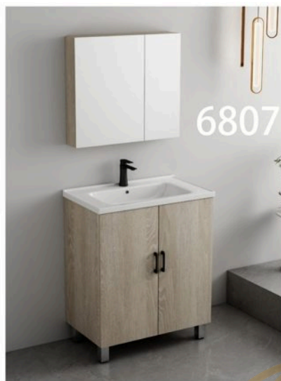
6807A-60 ( ¥: 2617 ) Main Cabinet: 600x480x800mm Mirror Cabinet: 550x130x700mm Material: Plywood+Ceramic Basin
